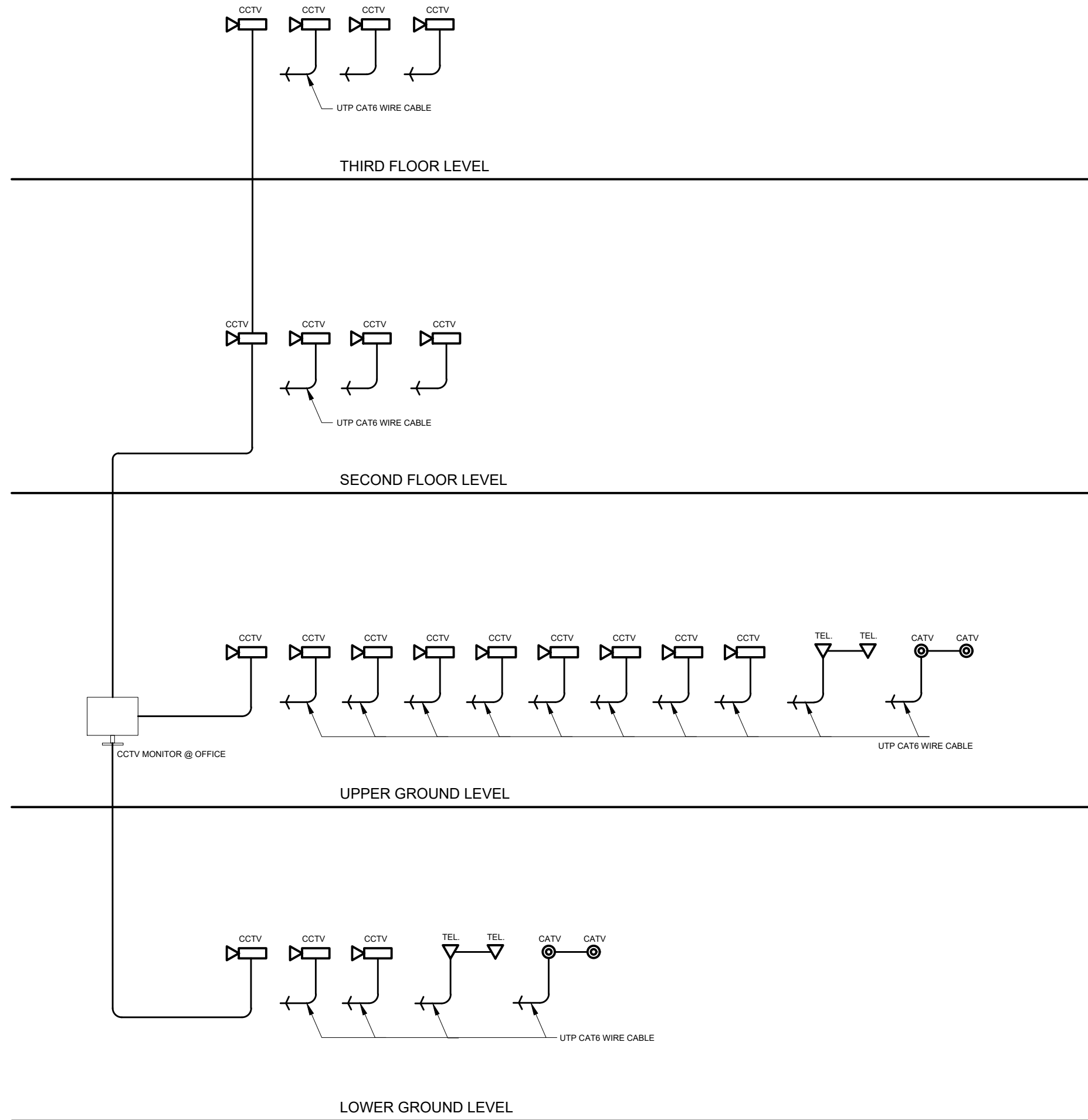
CCTV SINGLE LINE DIAGRAM
