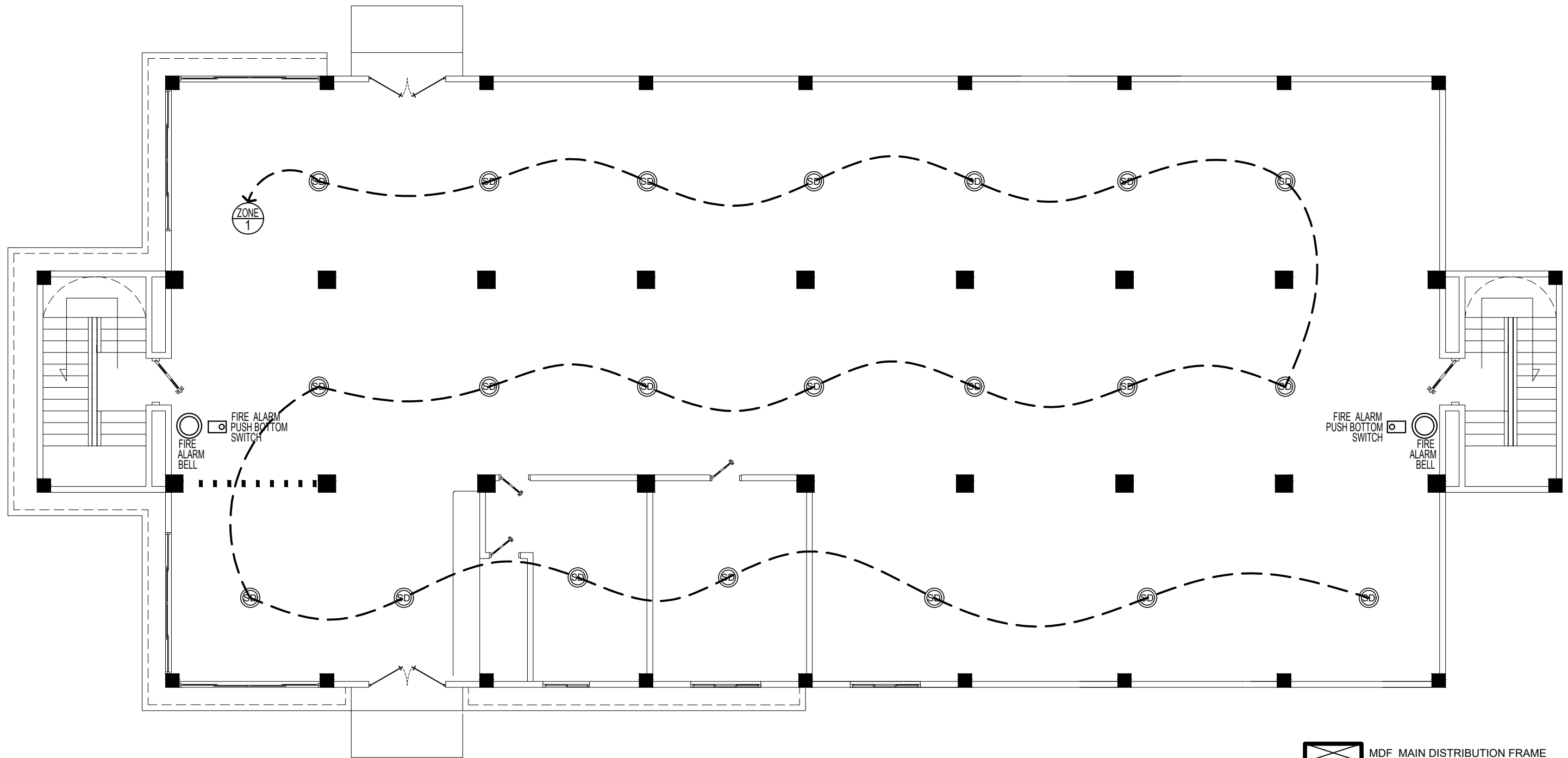
1 LOWER GROUND FLOOR LAYOUT(FDAS ) AUX-5 SCALE 1:100 M.
