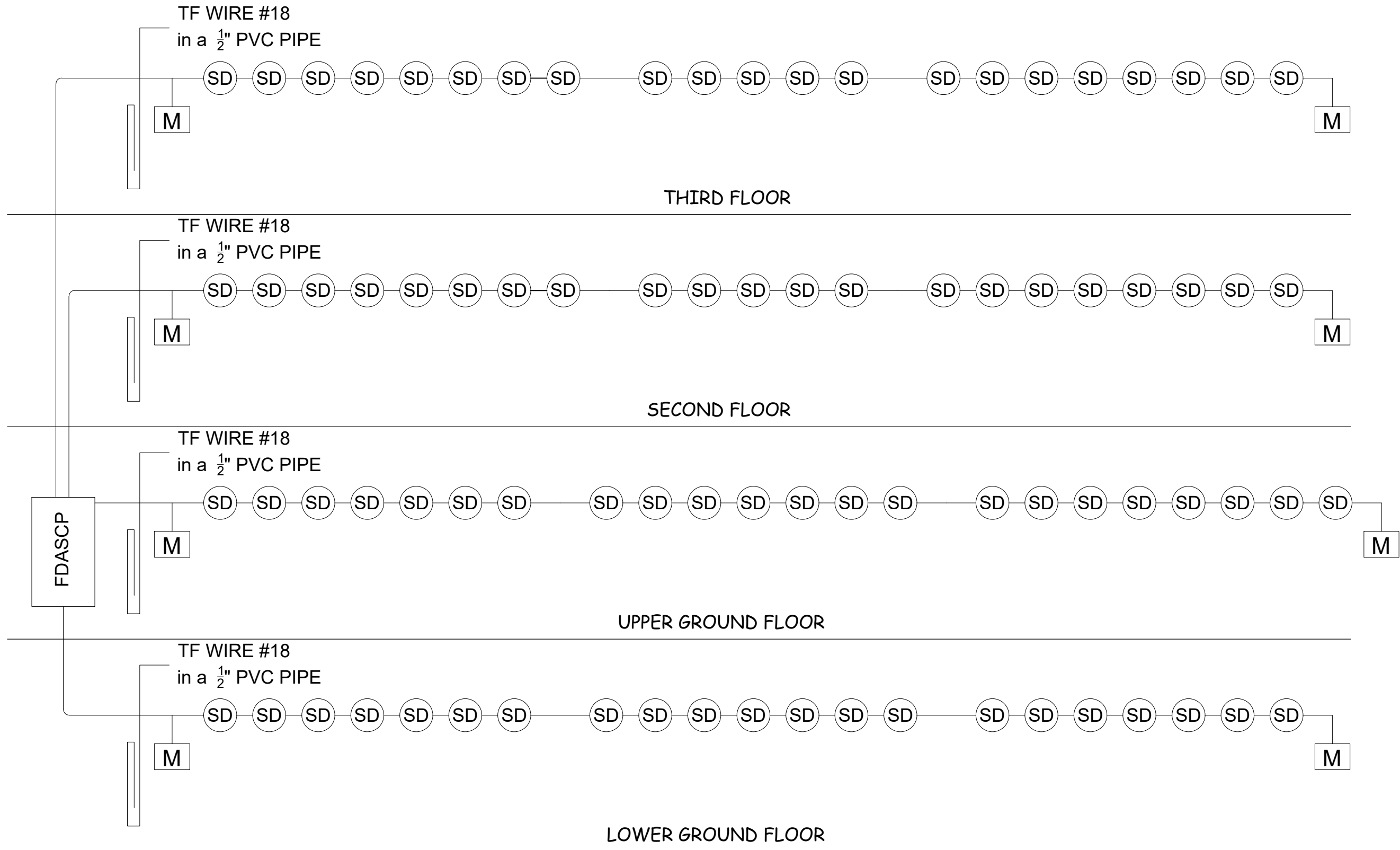
3 (FDAS) SINGLE LINE DIAGRAM AUX-5 SCALE NDTS
