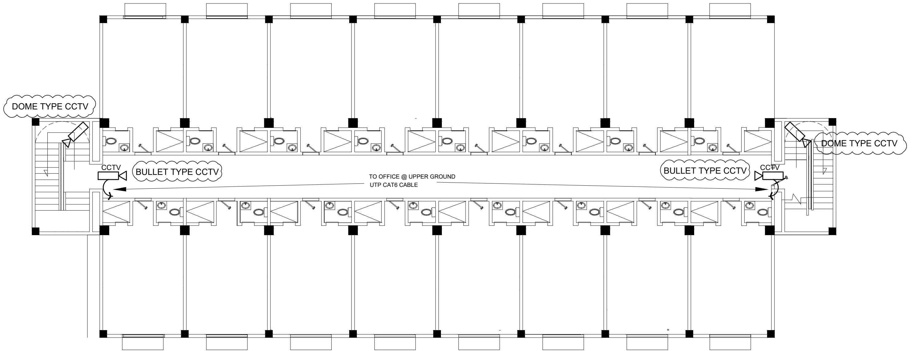
3 EE-6 SECOND FLOOR CCTV LAYOUT SCALE 1:100 M.
