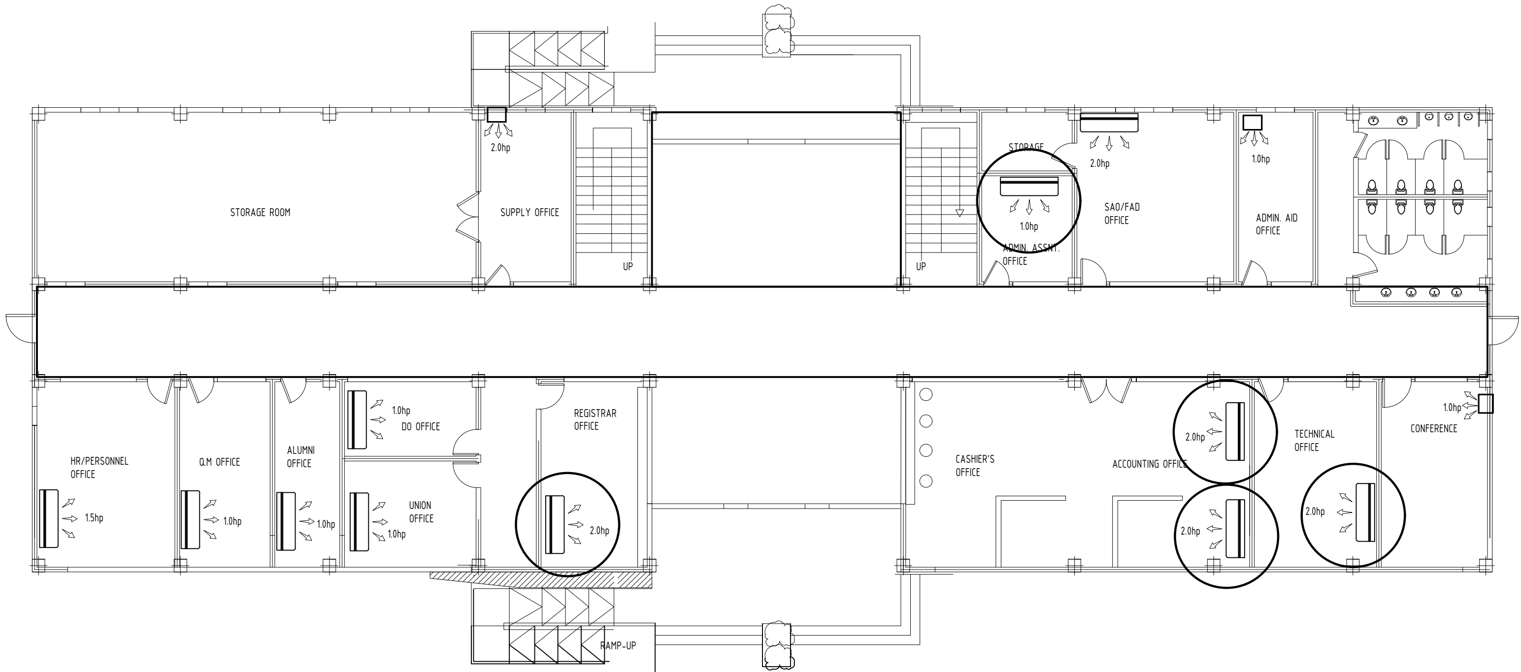
GROUND FLOOR AIR CONDITIONING LAY-OUT
