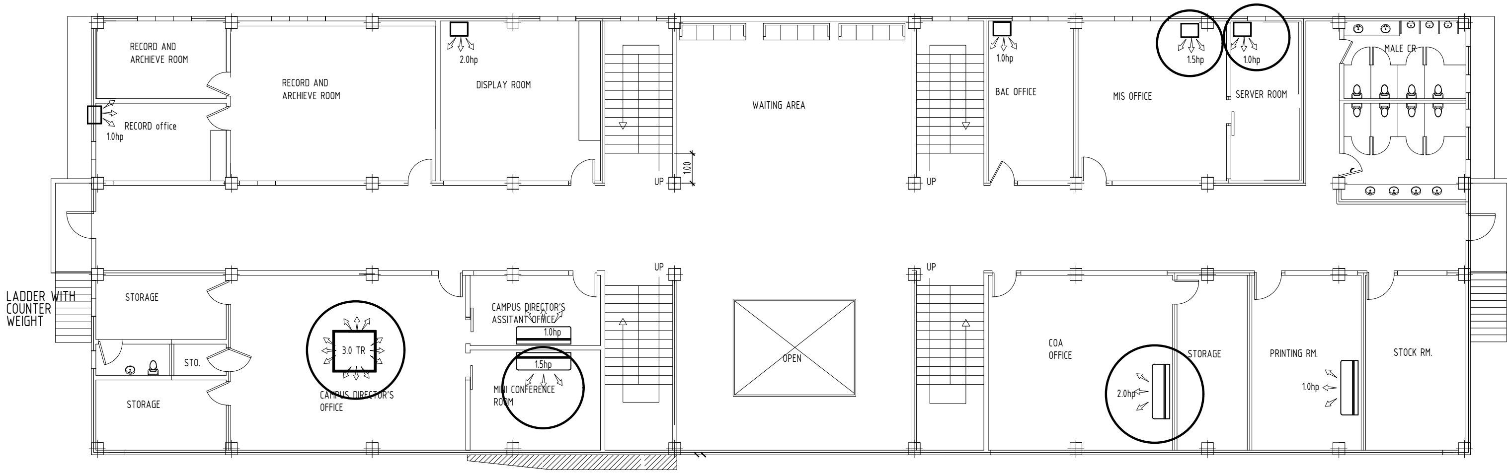
SECOND FLOOR AIR CONDITIONING LAY-OUT
