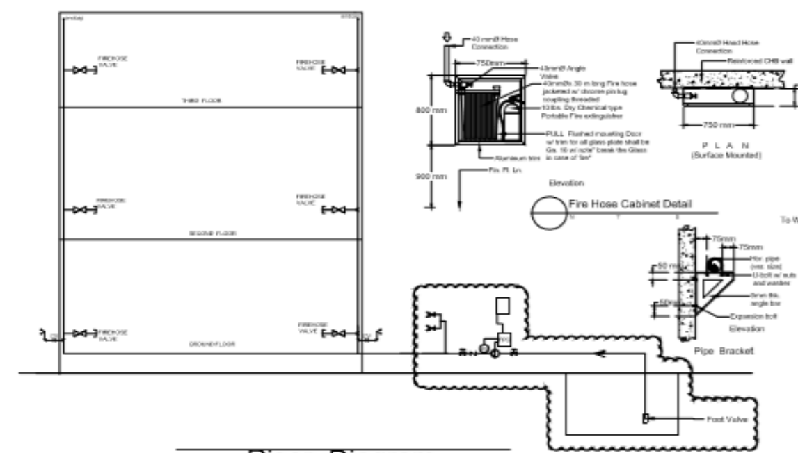
Riser Diagram
