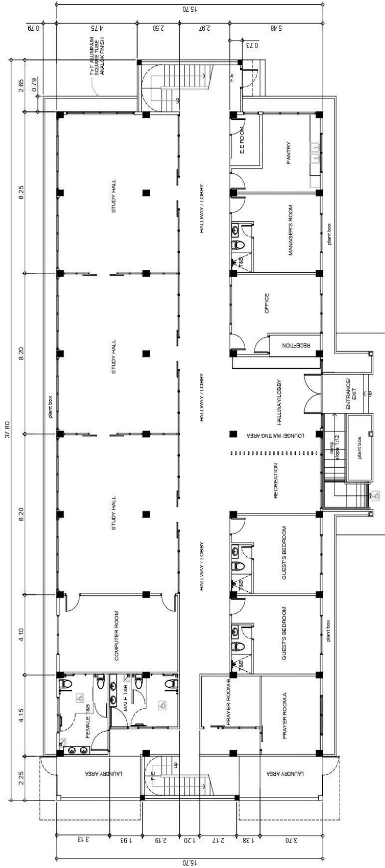
DORMITORY 2 GROUND FLOOR PLAN SCALE 1:100 METERS
